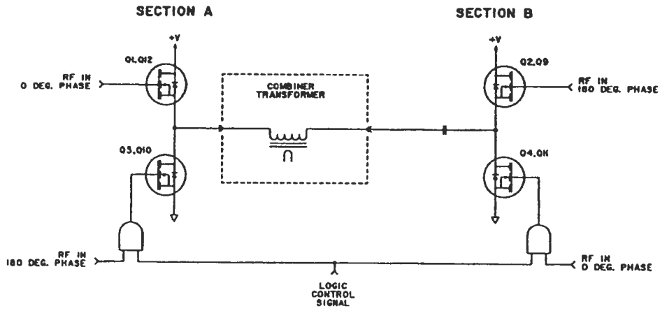
Figure C-1. RF Amplifier Module, Simplified Diagram
