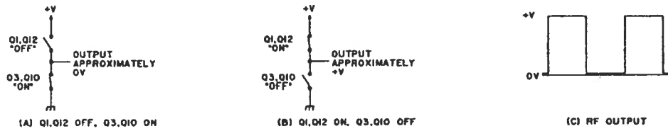
Figure C-2. RF Amplifier Operation, Half-Quad
