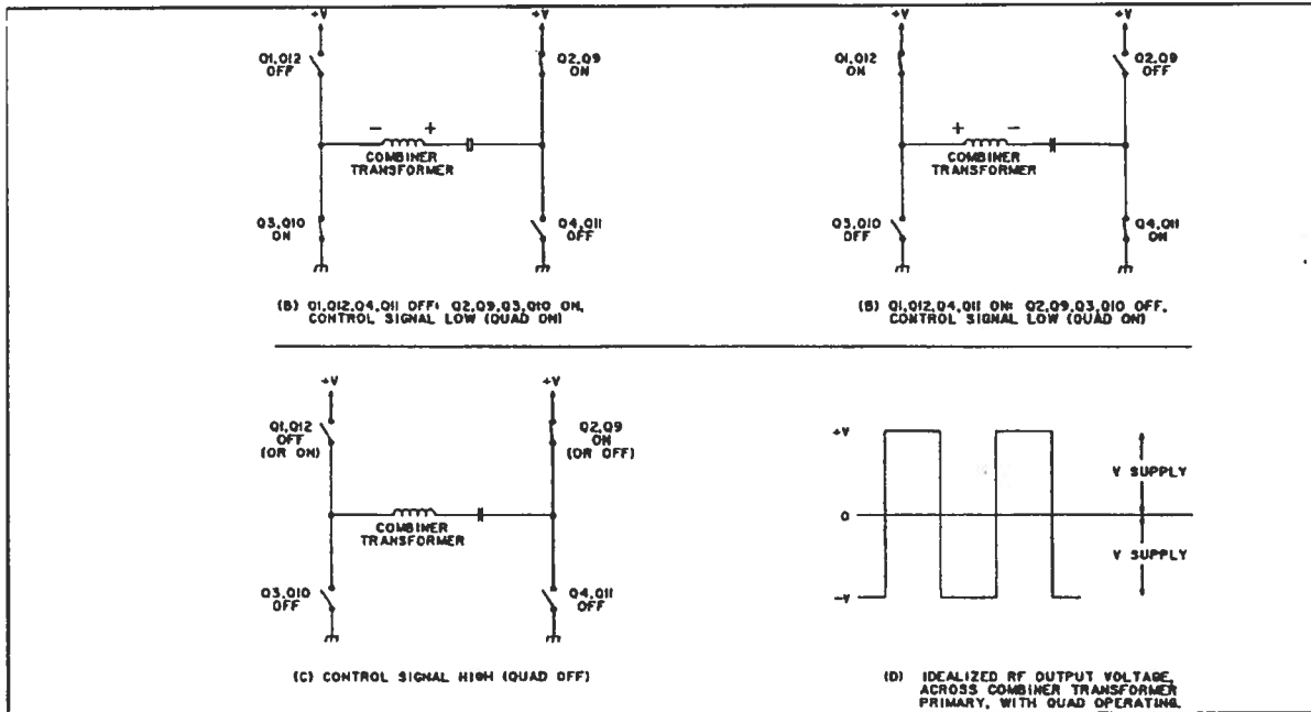
Figure C-3. RF Amplifier Operation, Full Quad
