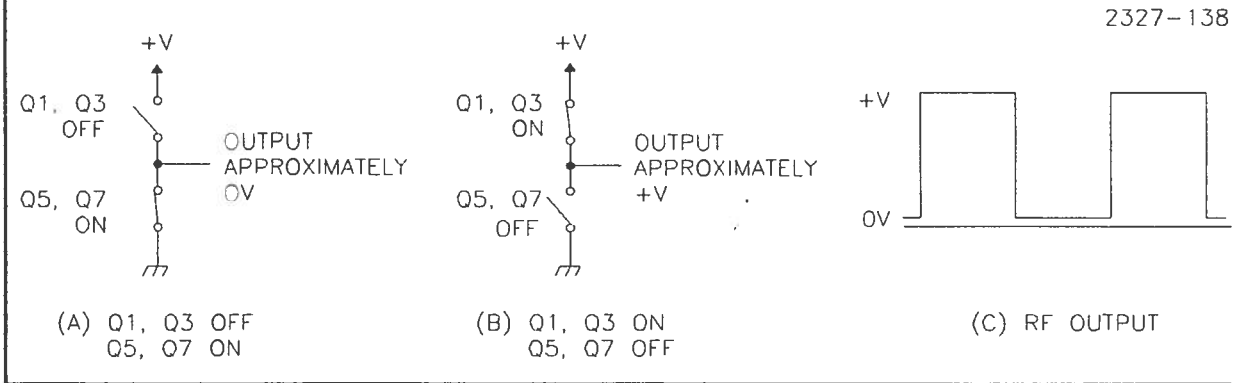
Figure G-3. RF Amplifier Half Quad Operation
